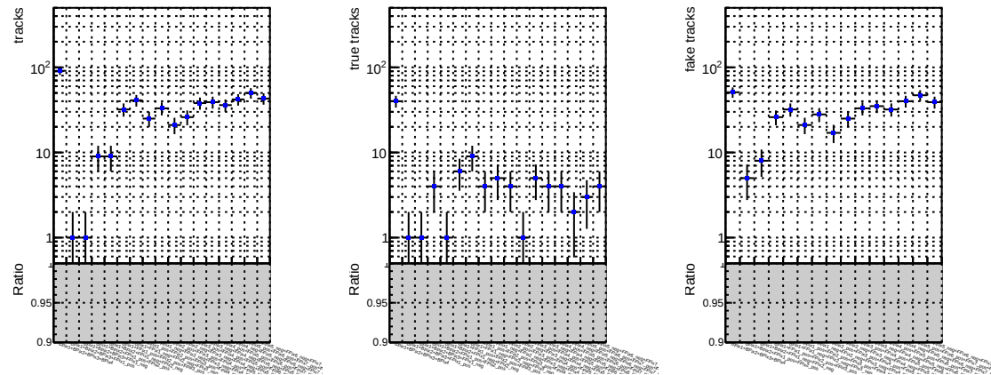
N of reco track vs. \chi^2 DQM_V0001_R000000001_Global_CMSSW_X_Y_Z_RECO
