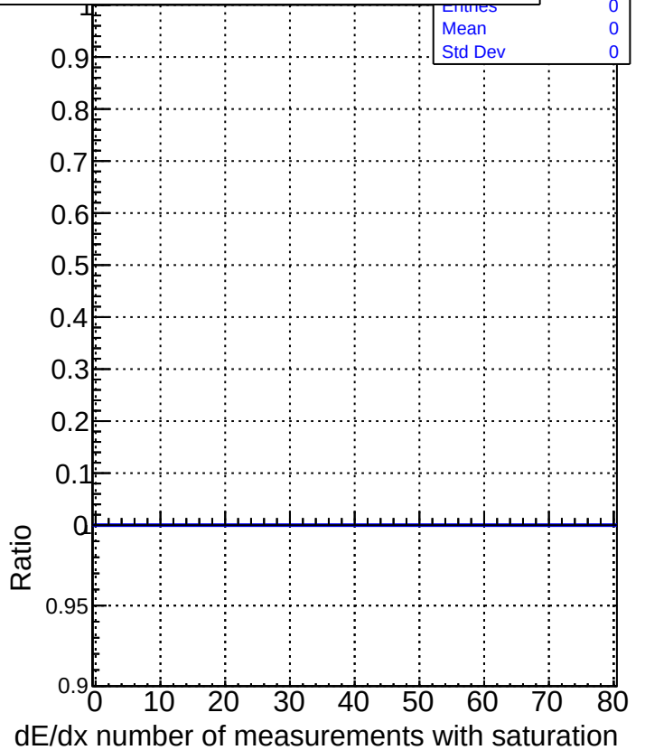
DQM_V0001_R000000001_Global_CMSSW_X_Y_Z_RECO
