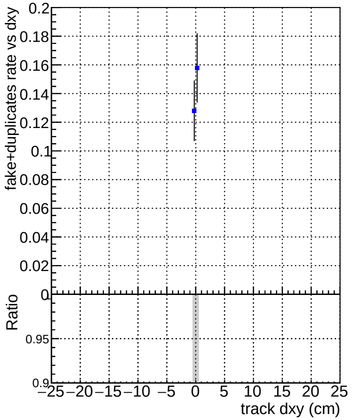
DQM_V0001_R000000001_Global_CMSSW_X_Y_Z_RECO
