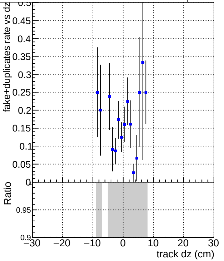
DQM_V0001_R000000001_Global_CMSSW_X_Y_Z_RECO
