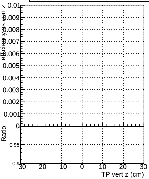
Efficiency vs TP vert r (cm) DQM_V0001_R000000001_Global_CMSSW_X.Y.Z_RECO
