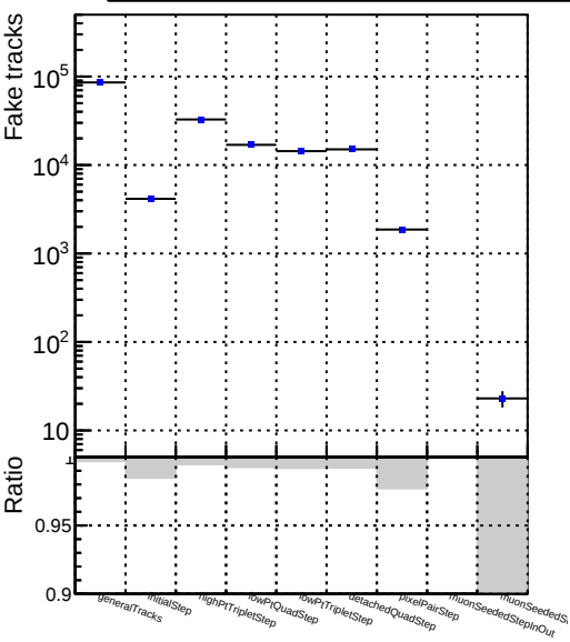
Number of DQM_V0001_R000000001_Global_CMSSW_X_Y_Z_RECO
