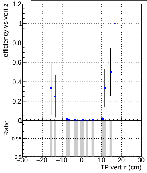
Efficiency vs. DQM_V0001_R000000001_Global_CMSSW_X_Y_Z_RECO
