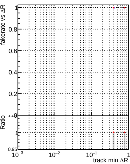
Fake rate vs ΔR(track, jet) DQM_mu_original DQM_mu_modified
