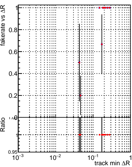
Fake rate vs \Delta R(\text{track, jet}) Legend: DQM_mu_original (grey line with blue dots), DQM_mu_modified (black line with red dots)
