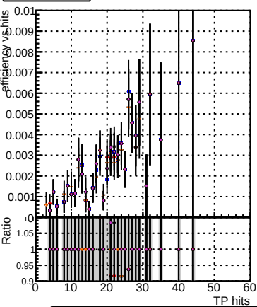
Efficiency vs TP hits DOM TT original DOM TT mod_models4 truthfinal_modelTEST-15 DOM TT mod_models4 truthallhits_modelTEST-12 DOM TT mod_models4 truthfinal_reg_modelTEST-12 DOM TT mod_models4 truthallhits_reg_modelTEST-11
