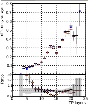
Efficiency vs hit Legend: DOM TT original DOM TT mod_models4 truthfinal_modelTEST-15 DOM TT mod_models4 truthhallhits_modelTEST-12 DOM TT mod_models4 truthfinal_reg_modelTEST-12 DOM TT mod_models4 truthhallhits_reg_modelTEST-11
