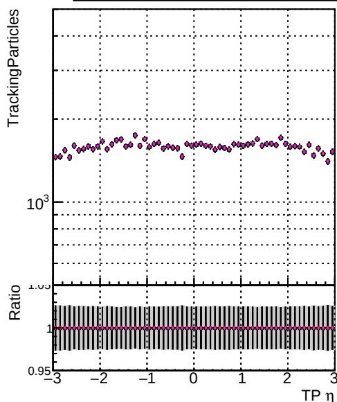
DOM TT mod model s4 truthallhits reg model TEST-12 DOM TT mod model s4 truthfinal reg model TEST-12 DOM TT mod model s4 truthallhits reg model TEST-11
