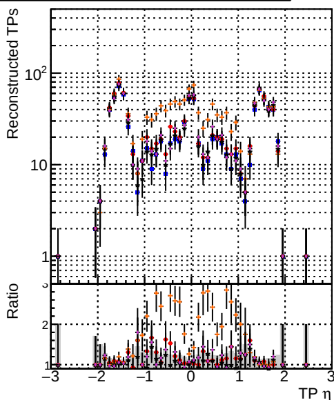
T-12 EST-12 ITEST-11
