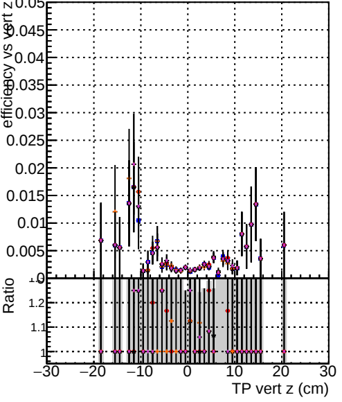
Efficiency vs TP vert z (cm) — original — mod models4 truthfinal — mod models4 truthfinal hits — mod models4 truthfinal reg — mod models4 truthfinal hits reg
