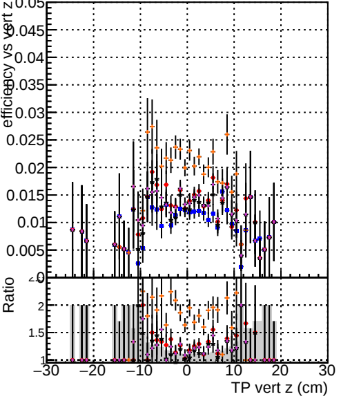
Efficiency vs TP vert z (cm) plot. The top panel shows efficiency (y-axis, 0 to 0.05) versus TP vert z (cm) (x-axis, linear scale from -30 to 30). The bottom panel shows the ratio (y-axis, 1 to 2) versus TP vert z (cm). The plot includes data points with error bars and a histogram. The data points are color-coded: black (original), blue (mod models4 truthfinal), orange (mod models4 truthfinal hits), red (mod models4 truthfinal reg), and purple (mod models4 truthfinal hits reg).
