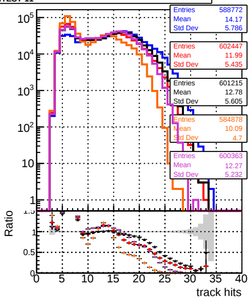
DQM TT original model s4 truthfinal modelTEST-15 DQM TT mod models4 truthfinal modelTEST-12 DQM TT mod models4 truthfinal hits modelTEST-12 DQM TT mod models4 truthfinal reg modelTEST-12 DQM TT mod models4 truthfinal hits reg modelTEST-11
