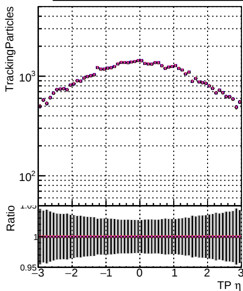
N of sin DOM TT mod mode s4 truthallhits reg model TEST-12 DOM TT mod mode s4 truthallhits reg model TEST-12 DOM TT mod mode s4 truthfinal reg model TEST-12 DOM TT mod mode s4 truthallhits reg model TEST-11
