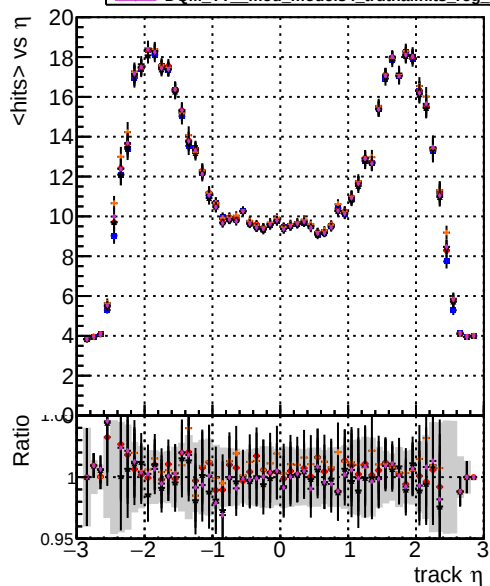
Legend for mean hits vs \eta : DOM TT original DOM TT mod models4 truthfinal DOM TT mod models4 truthfinal hits DOM TT mod models4 truthfinal reg DOM TT mod models4 truthfinal hits reg DOM TT mod models4 truthfinal reg modelTEST-12 DOM TT mod models4 truthfinal hits reg modelTEST-12 DOM TT mod models4 truthfinal hits reg modelTEST-11
