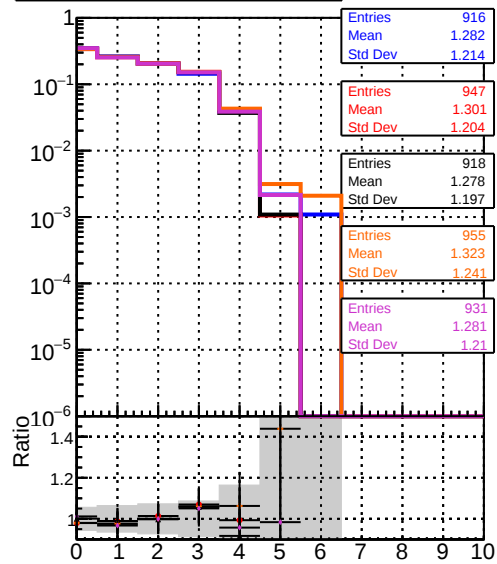
DOM TT original DOM TT mod models4 truthfinal modelTEST-15 DOM TT mod models4 truthfinalhits modelTEST-12 DOM TT mod models4 truthfinal reg modelTEST-12 DOM TT mod models4 truthfinalhits reg modelTEST-11
