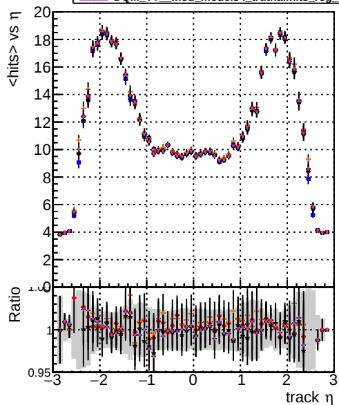
mean hit DOM TT original mod models4 truthfinal modelTEST-15 DOM TT original mod models4 truthfinalhits modelTEST-12 DOM TT original mod models4 truthfinal reg modelTEST-12 DOM TT original mod models4 truthfinalhits reg modelTEST-11
