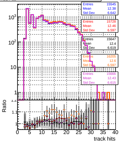
mean hit DOM TT original mod models4 truthfinal modelTEST-15 DOM TT original mod models4 truthfinalhits modelTEST-12 DOM TT original mod models4 truthfinal reg modelTEST-12 DOM TT original mod models4 truthfinalhits reg modelTEST-11
