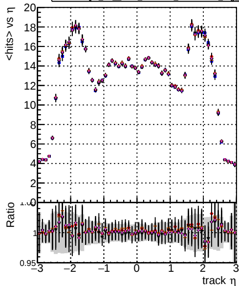
Legend for mean hits vs \eta : DOM TT original DOM TT mod models4 truthfinal modelTEST-15 DOM TT mod models4 truthfinal hits modelTEST-12 DOM TT mod models4 truthfinal reg modelTEST-12 DOM TT mod models4 truthfinal hits reg modelTEST-11
