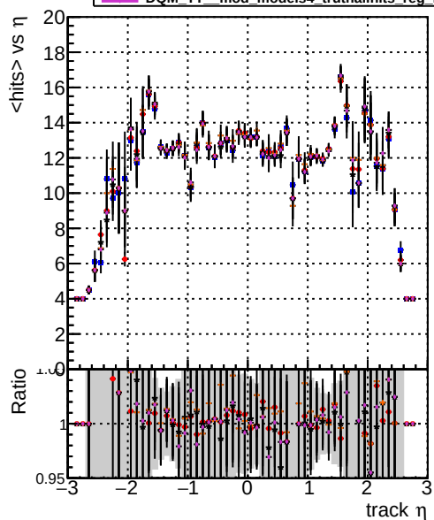
mean hits DQM TT original DQM TT mod models4 truthfinal DQM TT mod models4 truthfinal hits DQM TT mod models4 truthfinal reg DQM TT mod models4 truthfinal hits reg
