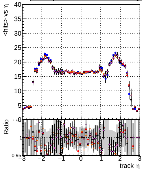
mean hit DOM TT original mod models4 truthfinal modelTEST-15 DOM TT mod models4 truthfinalhits modelTEST-12 DOM TT mod models4 truthfinal reg modelTEST-12 DOM TT mod models4 truthfinalhits reg modelTEST-11
