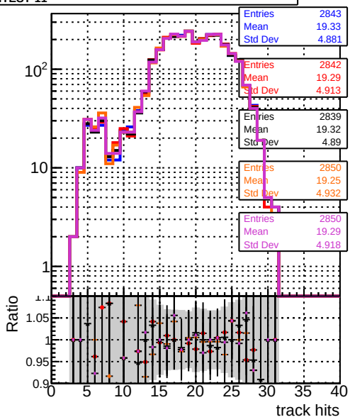
— DQM TT original — DQM TT mod models4 truthfinal modelTEST-15 — DQM TT mod models4 truthfinalhits modelTEST-12 — DQM TT mod models4 truthfinal reg modelTEST-12 — DQM TT mod models4 truthfinalhits reg modelTEST-11
