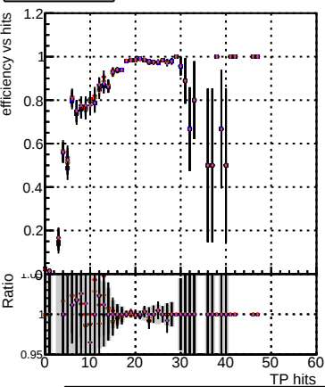
Efficiency vs TP hits Legend: DOM TT original DOM TT mod_models4 truthfinal_modelTEST-15 DOM TT mod_models4 truthhallhits_modelTEST-12 DOM TT mod_models4 truthfinal_reg_modelTEST-12 DOM TT mod_models4 truthhallhits_reg_modelTEST-11
