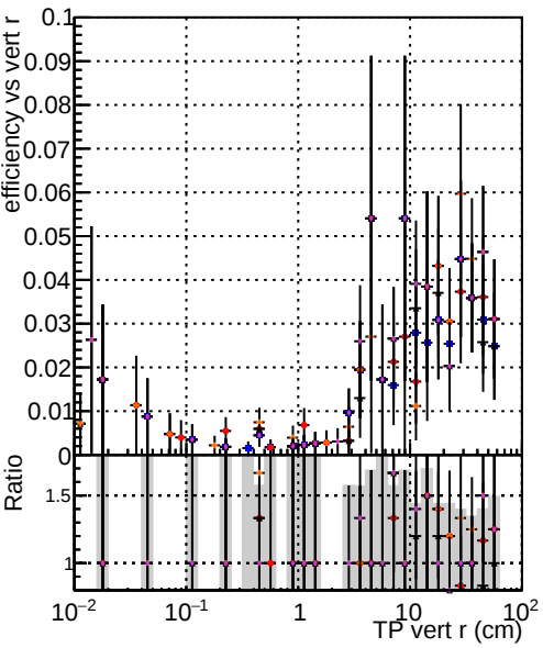
Efficiency vs. TP vert r (cm) DOM TT original mod models4 truthfinal modelTEST-15 DOM TT mod models4 truthfinal hits modelTEST-12 DOM TT mod models4 truthfinal reg modelTEST-12 DOM TT mod models4 truthfinal hits reg modelTEST-11
