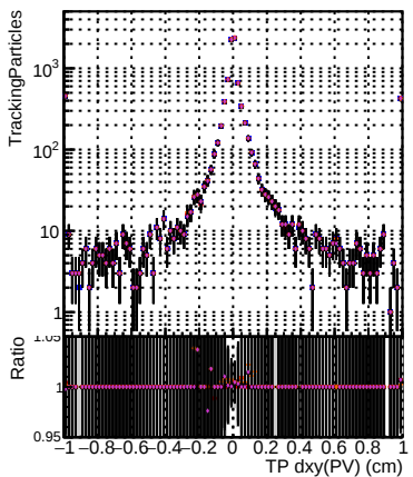
N of sim DOM TT original DOM TT mod_models4 truthfinal_modelTEST-15 DOM TT mod_models4 truthallhits_modelTEST-12 DOM TT mod_models4 truthfinal_reg_modelTEST-12 DOM TT mod_models4 truthallhits_reg_modelTEST-11
