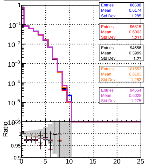
DQM TT original modelTEST-15 DQM TT mod models4 truthfinal modelTEST-12 DQM TT mod models4 truthfinal hits modelTEST-12 DQM TT mod models4 truthfinal reg modelTEST-12 DQM TT mod models4 truthfinal hits reg modelTEST-11
