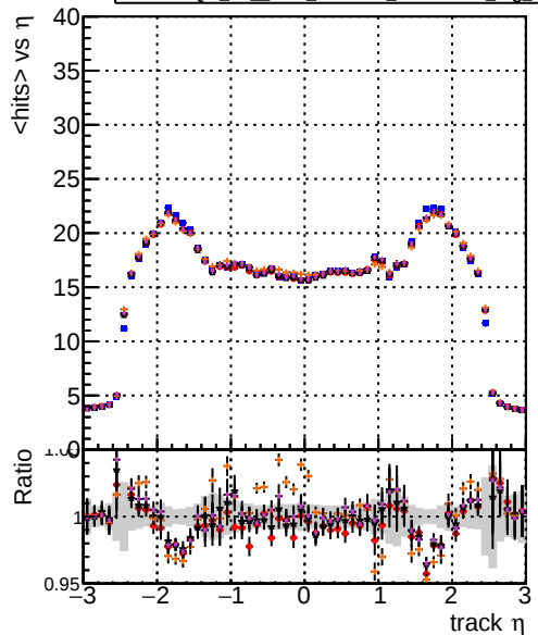
DOM TT original DOM TT mod models4 truthfinal modelTEST-15 DOM TT mod models4 truthfinal hits modelTEST-12 DOM TT mod models4 truthfinal reg modelTEST-12 DOM TT mod models4 truthfinal hits reg modelTEST-11
