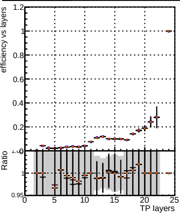
Efficiency vs hit Legend: DQM_TT_original DQM_TT_mod_modelsdeep_truthfinal_modelTEST-25 DQM_TT_mod_modelsdeep_truthfinal_reg_altmodelTEST-29 DQM_TT_mod_modelsdeep_truthfinal_reg_modelTEST-24
