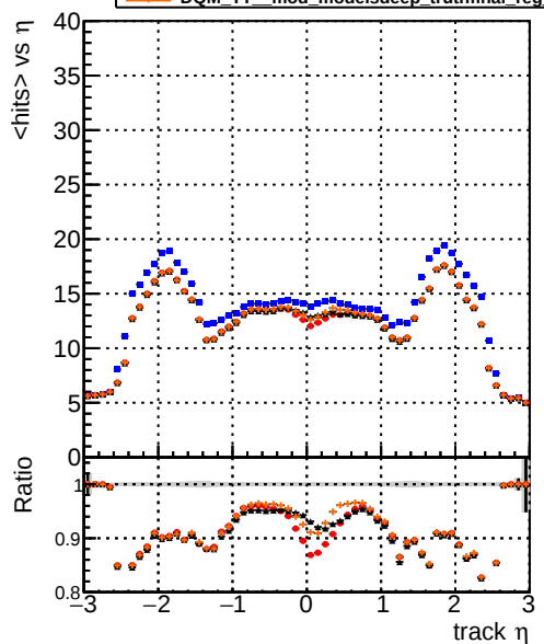
mean hits vs \eta Legend: DOM TT original DOM TT mod_modeldeep_truthfinal_modelTEST-25 DOM TT mod_modeldeep_truthfinal_reg_altmodelTEST-29 DOM TT mod_modeldeep_truthfinal_reg_modelTEST-24
