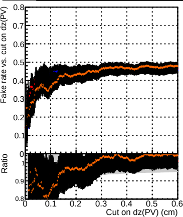
Fake rate Legend: DQM TT original DQM TT mod_modeldeep_truthfinal_modelTEST-25 DQM TT mod_modeldeep_truthfinal_reg_altmodelTEST-29 DQM TT mod_modeldeep_truthfinal_reg_modelTEST-24
