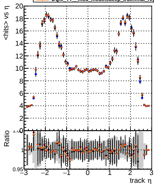
mean hits vs \eta DQM TT original DQM TT mod_modeldeep_truthfinal_modelTEST-25 DQM TT mod_modeldeep_truthfinal_reg_altmodelTEST-29 DQM TT mod_modeldeep_truthfinal_reg_modelTEST-24
