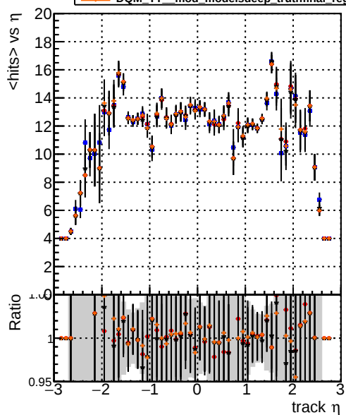
mean hit DQM TT original DQM TT mod_modelstdeep_truthfinal_modelTEST-25 DQM TT mod_modelstdeep_truthfinal_reg_modelTEST-29 DQM TT mod_modelstdeep_truthfinal_reg_modelTEST-24
