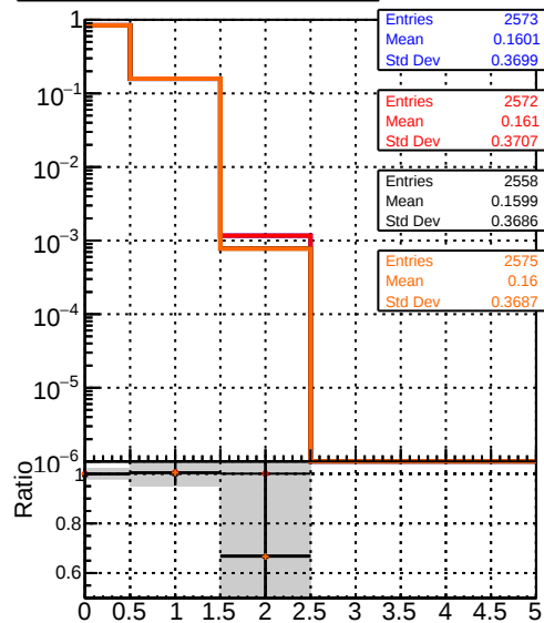
mean hit DQM TT original DQM TT mod_modelstdeep_truthfinal_modelTEST-25 DQM TT mod_modelstdeep_truthfinal_reg_modelTEST-29 DQM TT mod_modelstdeep_truthfinal_reg_modelTEST-24
