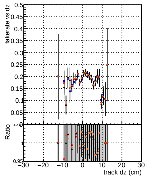
Fake rate vs dz Legend: - Blue line: DOM II original - Red line: DOM II mod model - Green line: DOM II deep truth final model - Black line: DOM II TEST-25 - Orange line: DOM II TEST-29 - Grey line: DOM II TEST-24
