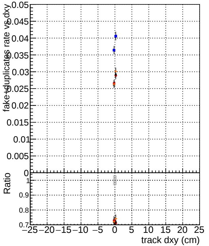
Legend for the bottom plot: DQM_TT_original DQM_TT_mod_modelsdeep_truthfinal_modelTEST-25 DQM_TT_mod_modelsdeep_truthfinal_reg_altmodelTEST-29 DQM_TT_mod_modelsdeep_truthfinal_reg_modelTEST-24
