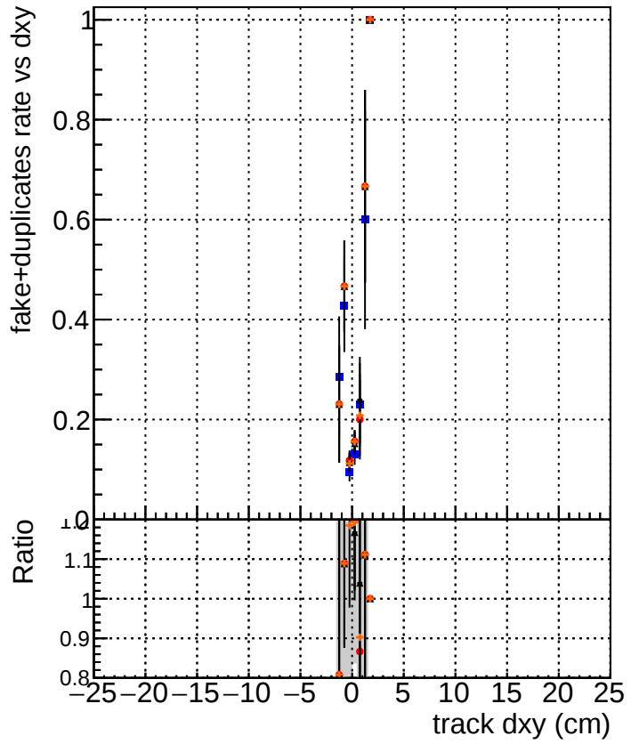
DQM_TT_original DQM_TT_mod_modelsdeep_truthfinal_modelTEST-25 DQM_TT_mod_modelsdeep_truthfinal_reg_altmodelTEST-29 DQM_TT_mod_modelsdeep_truthfinal_reg_modelTEST-24
