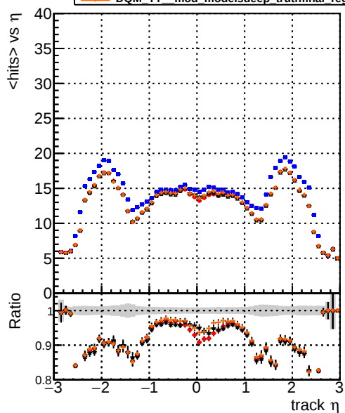
mean hit DQM TT original DQM TT mod_modeldeep_truthfinal_modelTEST-25 DQM TT mod_modeldeep_truthfinal_reg_modelTEST-24 DQM TT mod_modeldeep_truthfinal_reg_modelTEST-24
