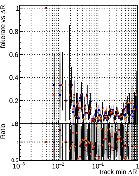
Fake rate vs \Delta R(\text{track, jet}) Legend: original (black) mod (blue) deep (red) truthfinal (orange) reg (grey) Model names: TEST-25, TEST-29, TEST-24
