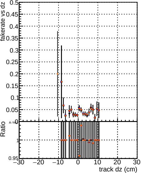
Fake rate vs dz Legend: DOM IT original, DOM IT mod model, deep truth final model, TEST-25, TEST-29, TEST-24
