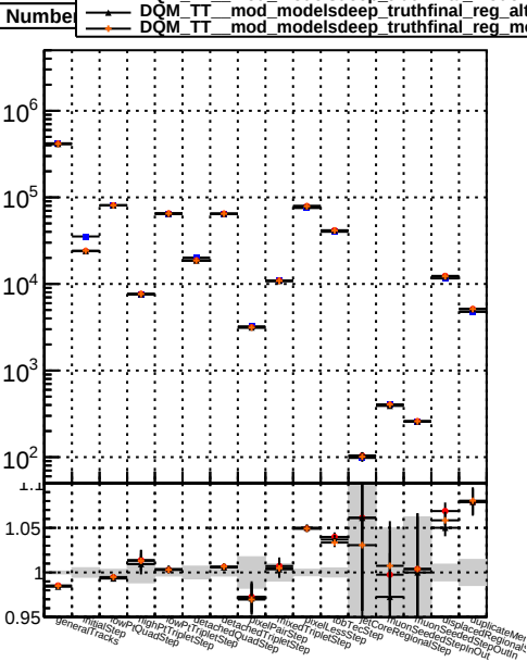
Number of pileup tracks vs collection
