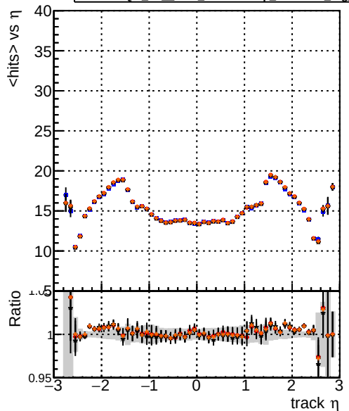
mean hits vs \eta Legend: - DQM TT original (blue line) - DQM TT mod_modeldeep_truthfinal_modelTEST-25 (red line) - DQM TT mod_modeldeep_truthfinal_reg_altmodelTEST-29 (black line) - DQM TT mod_modeldeep_truthfinal_reg_modelTEST-24 (orange line)
