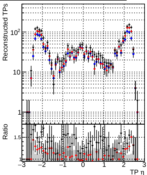
● DQM_TT_original ● DQM_TT_mod_modelsdeep_truthfinal_reg_modelTEST-24 ● DQM_TT_mod_modelsdeep_cumulativevetest
