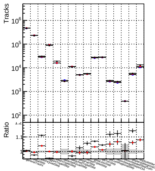
—●— DQM_TT_mod_modelsdeep_truthfinal_reg_modelTEST-24 —▲— DQM_TT_mod_modelsdeep_cumulativetest
