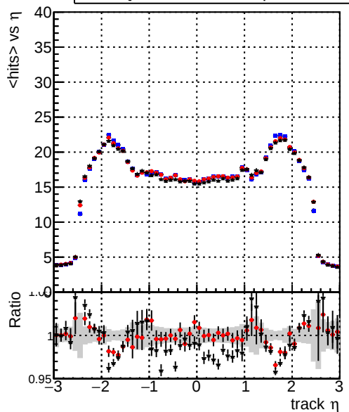
mean hits vs \eta — DQM_TT_original — DQM_TT_mod_modelsdeep_truthfinal_reg_modelTEST-24 — DQM_TT_mod_modelsdeep_cumulativevetest
