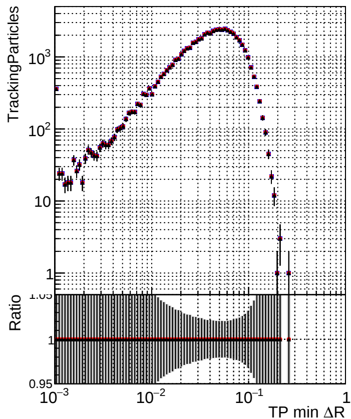
N of simulated tracks vs TP \Delta R (TP, jet) DQM_TT_original DQM_TT_mod_modelsdeep_truthfinal_reg_modelTEST-24 DQM_TT_mod_modelsdeep_cumulativetest
