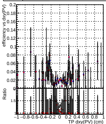
Efficienc → DQM_TT_mod_modelsdeep_cumulativetest
