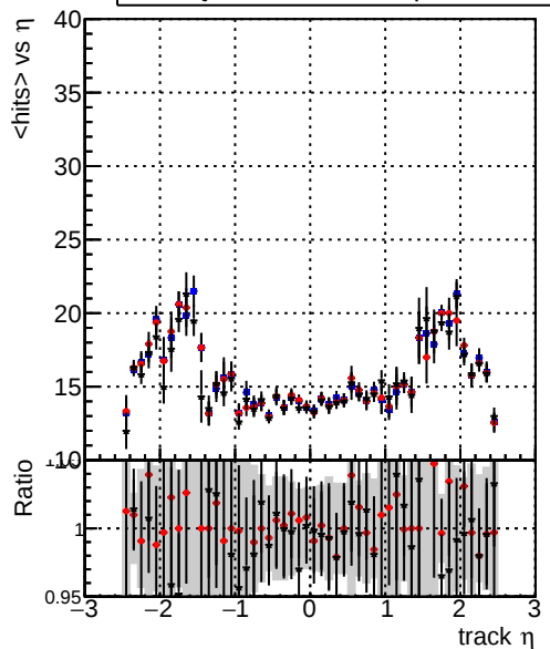
mean hits vs \eta — DQM_TT_original — DQM_TT_mod_modelsdeep_truthfinal_reg_modelTEST-24 — DQM_TT_mod_modelsdeep_cumulativetest
