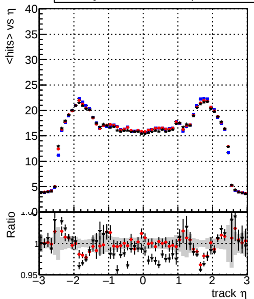
mean hits — DQM_TT_original — DQM_TT_mod_modelsdeep_truthfinal_reg_modelTEST-24 — DQM_TT_mod_modelsdeep_cumulativevetest
