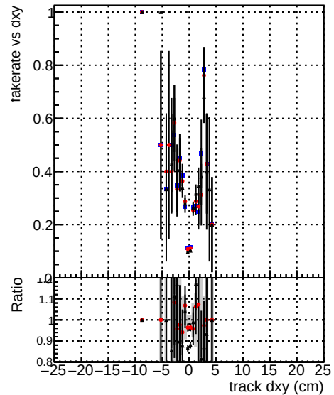
DOM TT original DOM TT mod modeldeep truthfinal reg_modelTEST-24 DOM TT mod modeldeep cumulativetest
