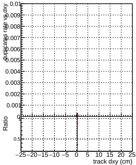
DOM TT original DOM TT mod modeldeep truthfinal reg_modelTEST-24 DOM TT mod modeldeep cumulativetest
