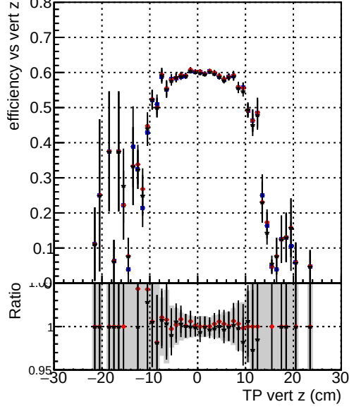
Efficiency vs. sim PV z — DQM_TT_original — DQM_TT_mod_modelsddeep_truthfinal_reg_modelTEST-24 — DQM_TT_mod_modelsddeep_cumulativetest
