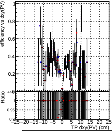
Efficiency vs Dxy(PV) Legend: DQM_TT_original (blue squares) DQM_TT_mod_modelsdeep_truthfinal_reg_modelTEST-24 (red circles) DQM_TT_mod_modelsdeep_cumulativetest (black circles)
